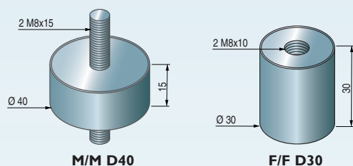
ANTIVIBRATION FIXING
